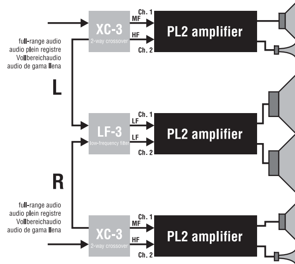
3-way system
