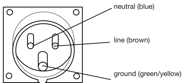
Figure 2.3. IEC 309 power connector pin-out
