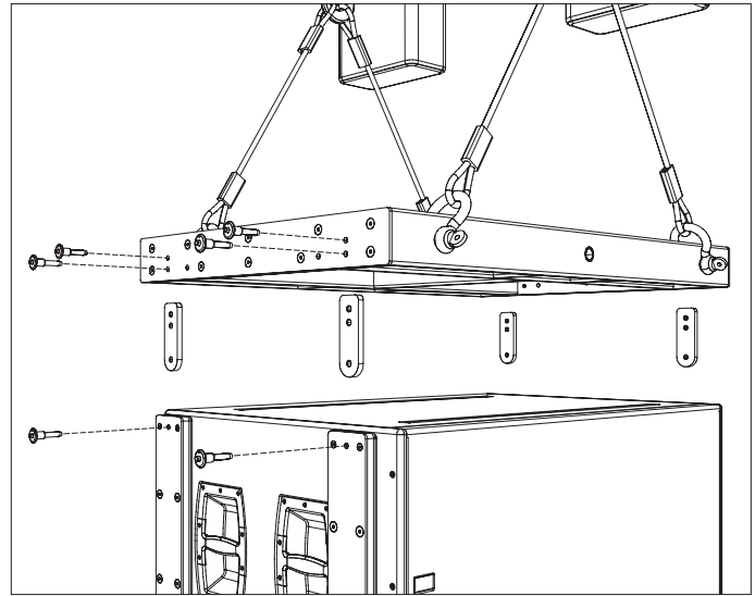
Figure 7.4. Multiple 700-HP subwoofers can be supported by the MTG-700 multipurpose grid.
