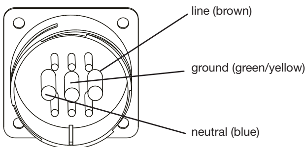
Figure 2.4. VEAM multipin connector power pin-out
