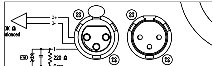
Figure 3.2. 700-HP rear panel audio input connectors
