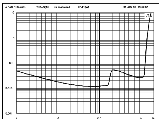
MF24: Total harmonic distortion versus output power, into 4Ω, at 1 KHz.
