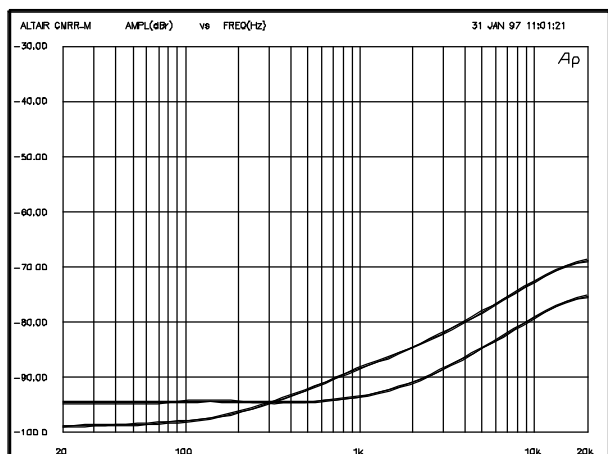
MF24: Typical common mode relation ratio (C.M.R.) versus frequency.
