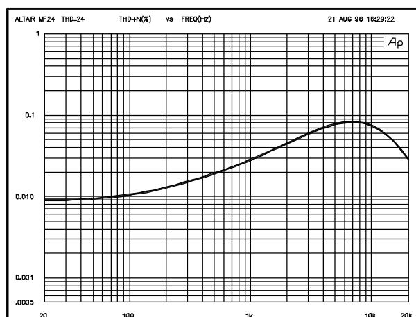
MF24: Total harmonic distortion versus frequency at rated output power, into 4Ω.
